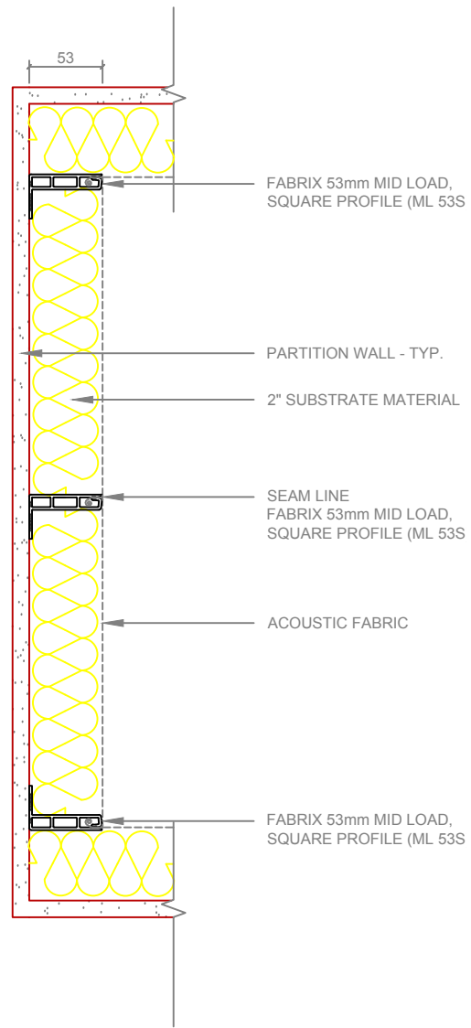
DTL 03 INSIDE CORNER SCALE 1:5
