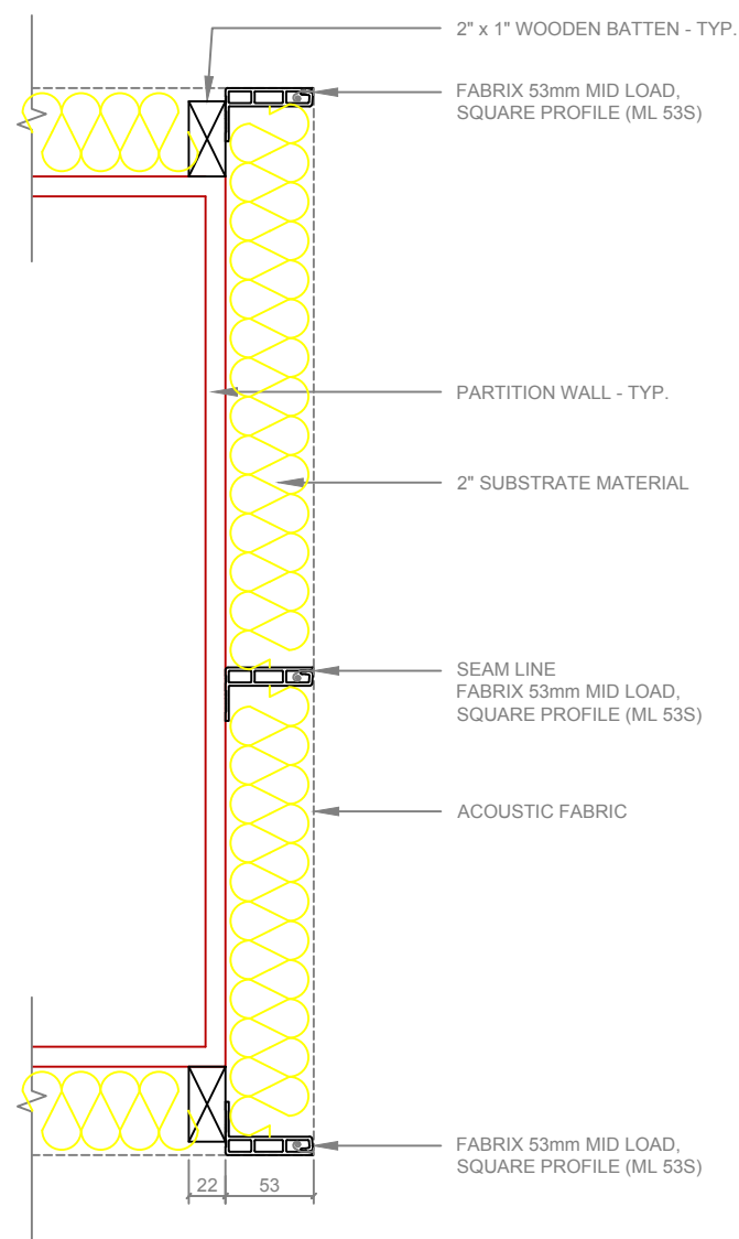
DTL 04 OUTSIDE CORNER WITH ML 53S SCALE 1:5
