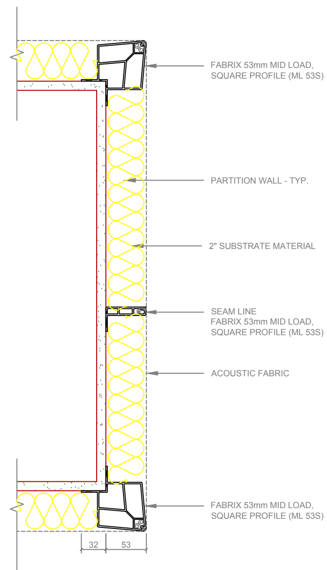
DTL 04 OUTSIDE CORNER WITH CL 53S SCALE 1:5
